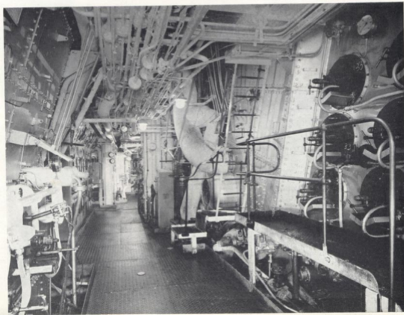
A glimpse below decks. The Windsor Castle is powered by twin screw double reduction high pressure turbines of pametrada design supplied with steam from three Babcock & Wilcox selectable superheat boilers having steam conditions of 600 lb. per square inch and 950°F., fitted with fully automatic combustion control
